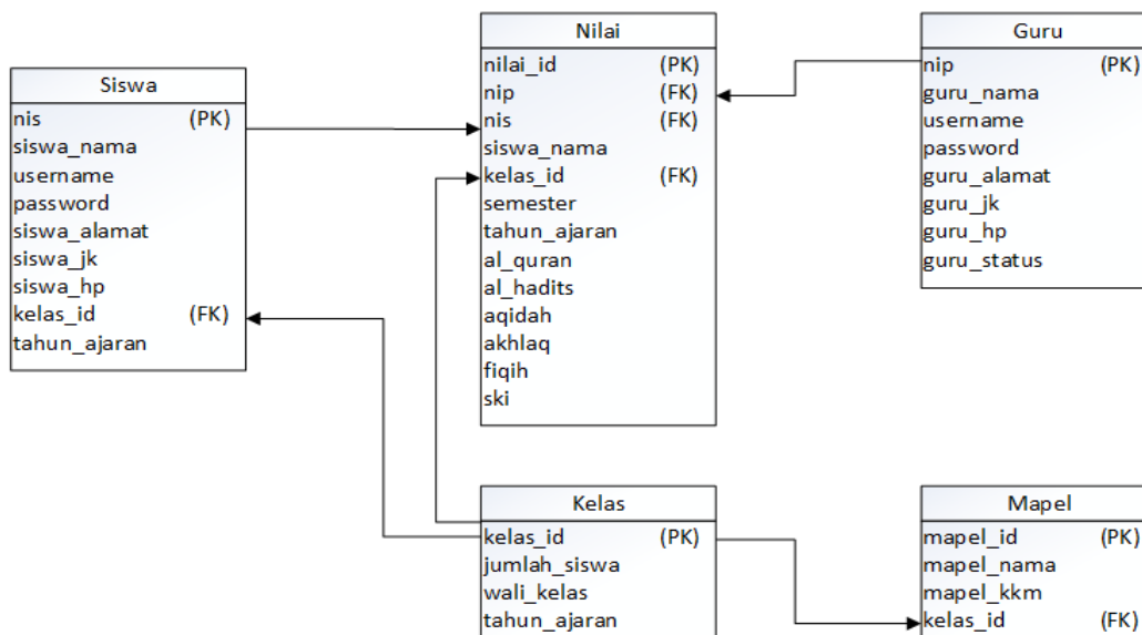
Gambar 2 Logical Relationship Structure Sistem Pengelohan Nilai Siswa
