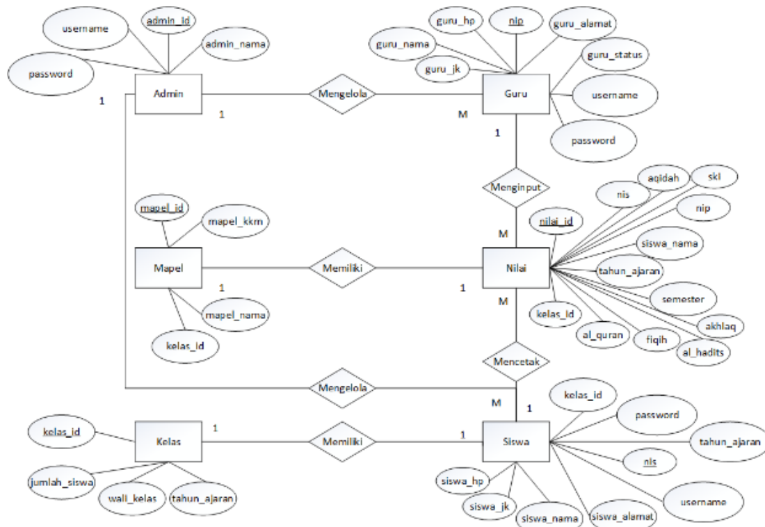
Gambar 1 Entity Relationship Diagram Sistem Pengelohan Nilai Siswa
