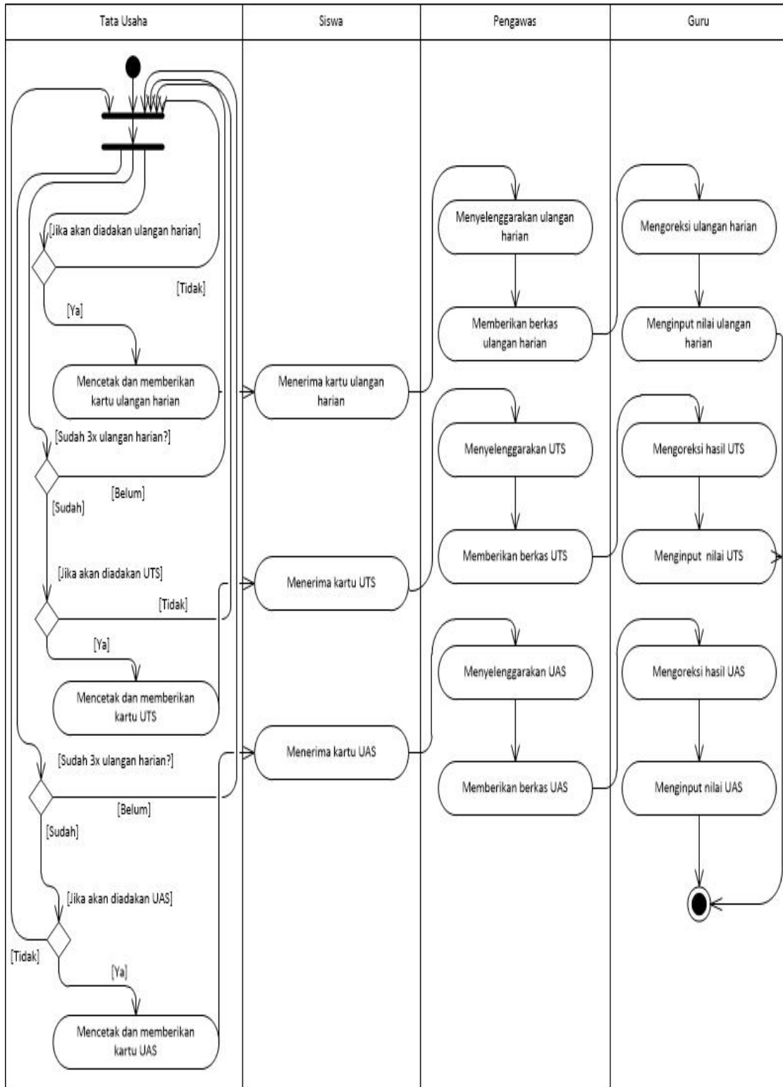
Gambar 2. Activity Diagram Proses Ujian (Ulangan Harian, UTS, UAS)
