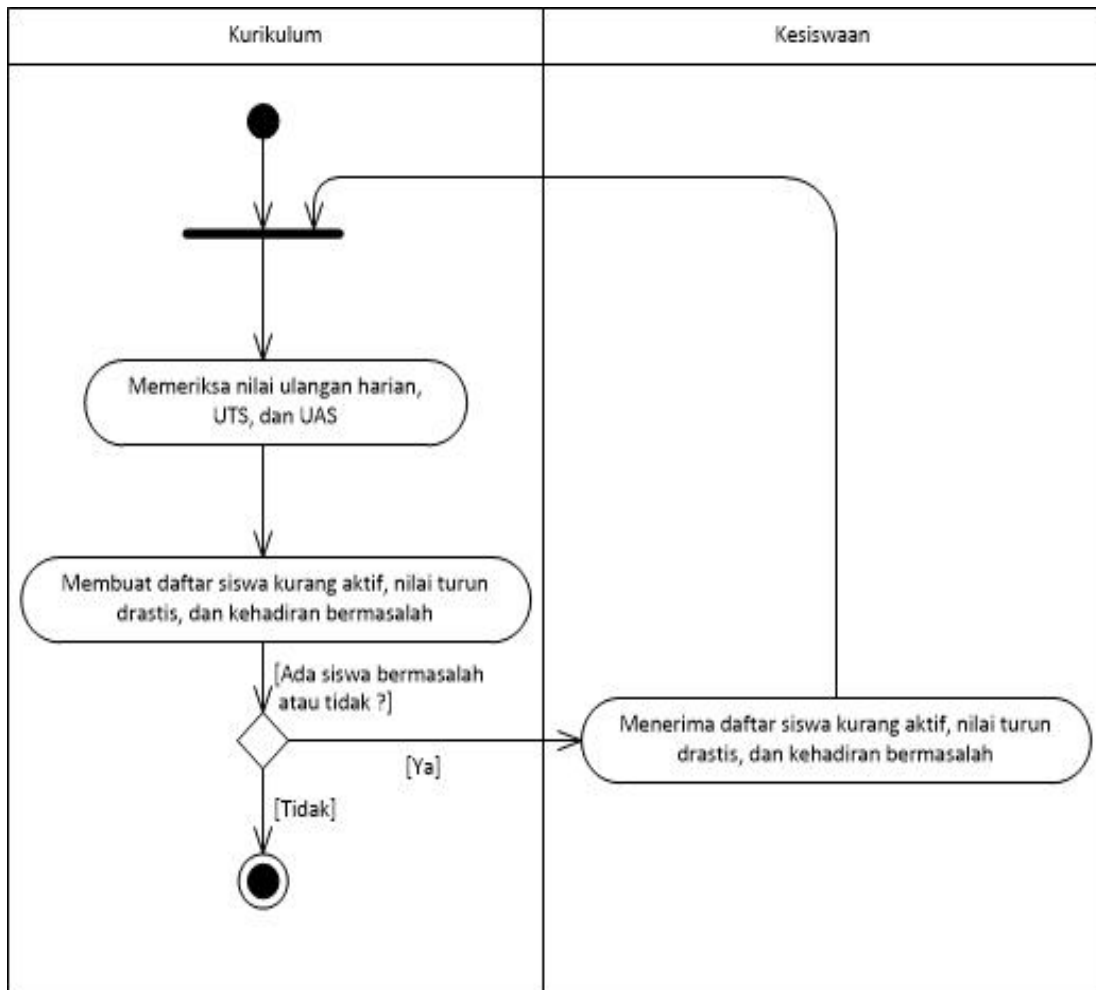
Gambar 3. Activity Diagram Proses Penilaian Siswa
