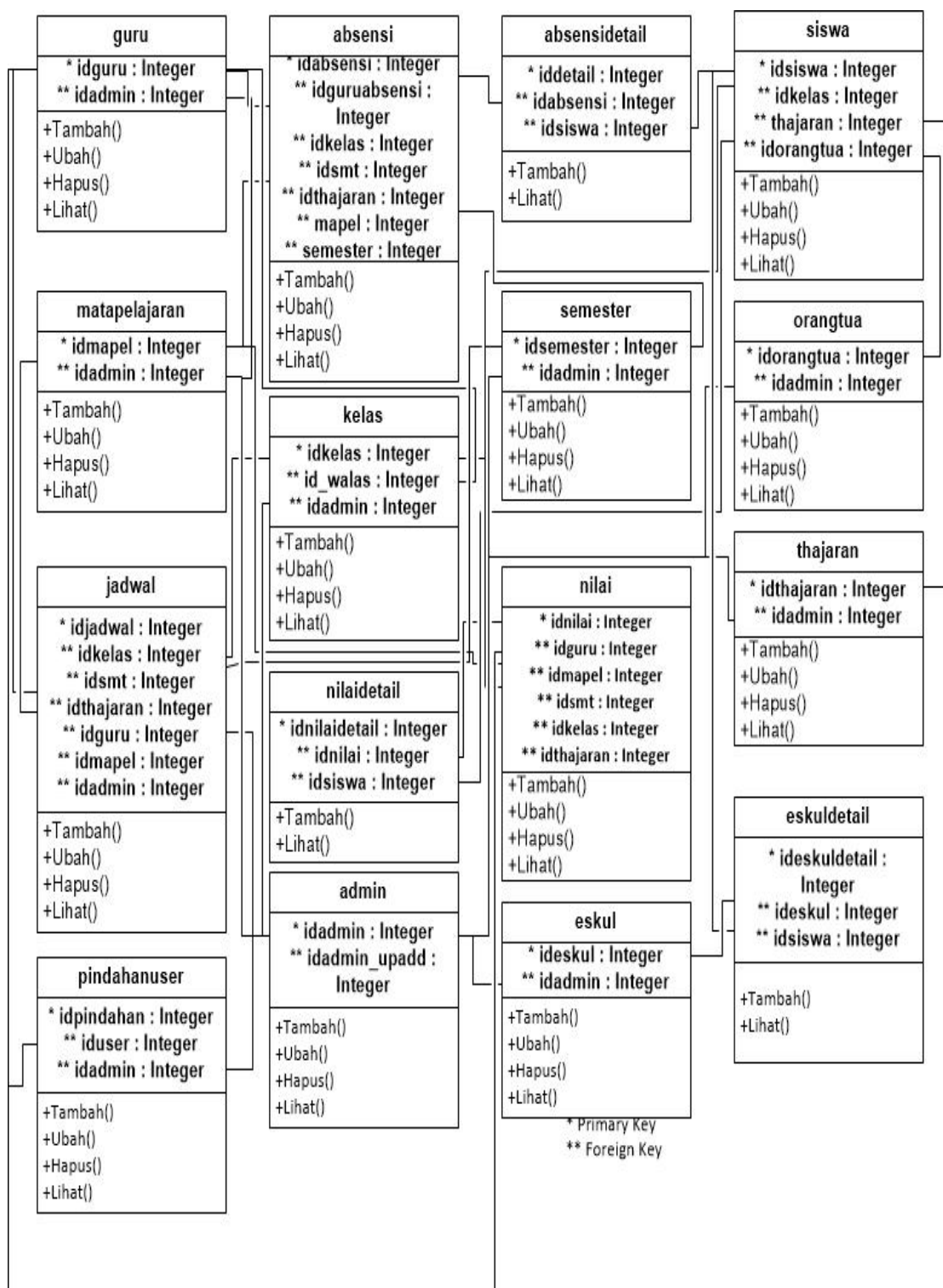
Gambar 14. Class Diagram
