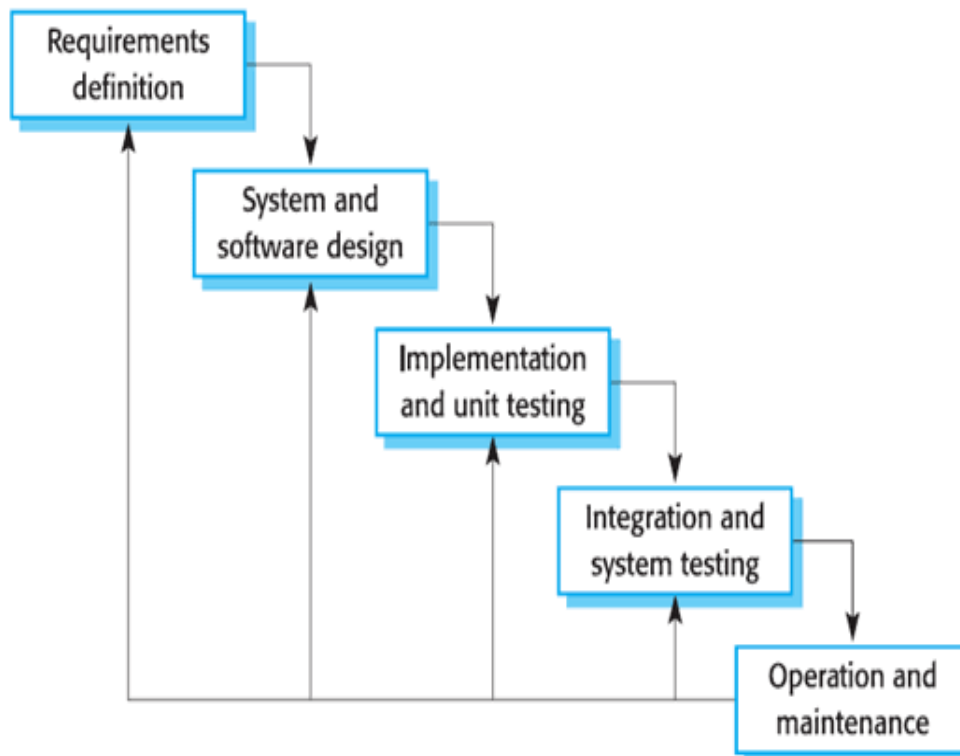
Gambar 1. Metode Waterfall
