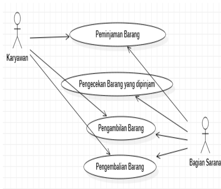
Gambar 2. Usecase diagram
